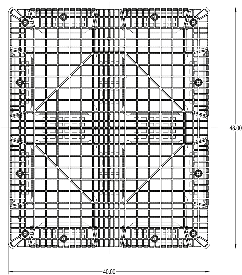
TOP VIEW
